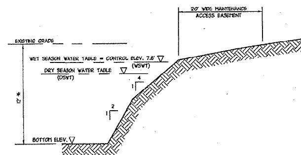
TYPICAL LAKE SECTION
